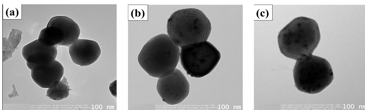
Fig. 3. TEM images of obtained (a) SrTiO 3 @Al and (b,c) obtained cocatalyst loaded SrTiO 3 @Al samples.
