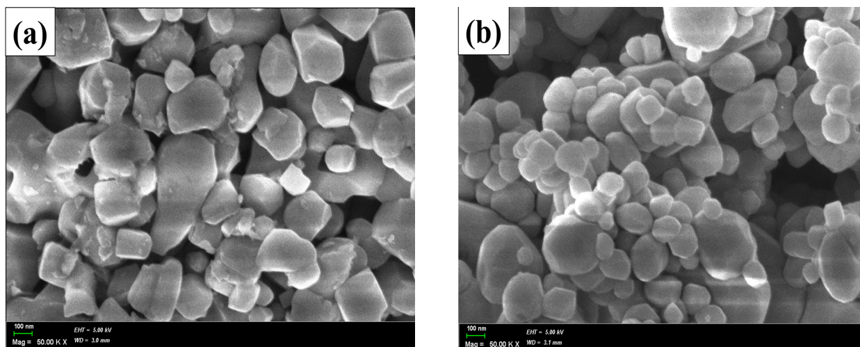
Fig. 1. SEM images of obtained (a) SrTiO 3 and (b) SrTiO 3 @Al.
