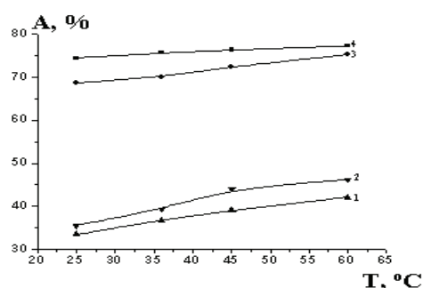
Fig. 6. Dependence of sorption CPB by composite gels on temperature: [MBAA] = 0.25%; [PPS] = 1 mol.%; C CPB = 1·10 -4 mole; BC:PAAm = 10:3 (4); 10:1 (3); BC:PHEA = 10:3 (2); 10:1 (1).
