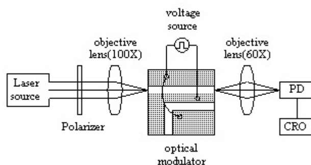
Fig. 6. Measurement system.
