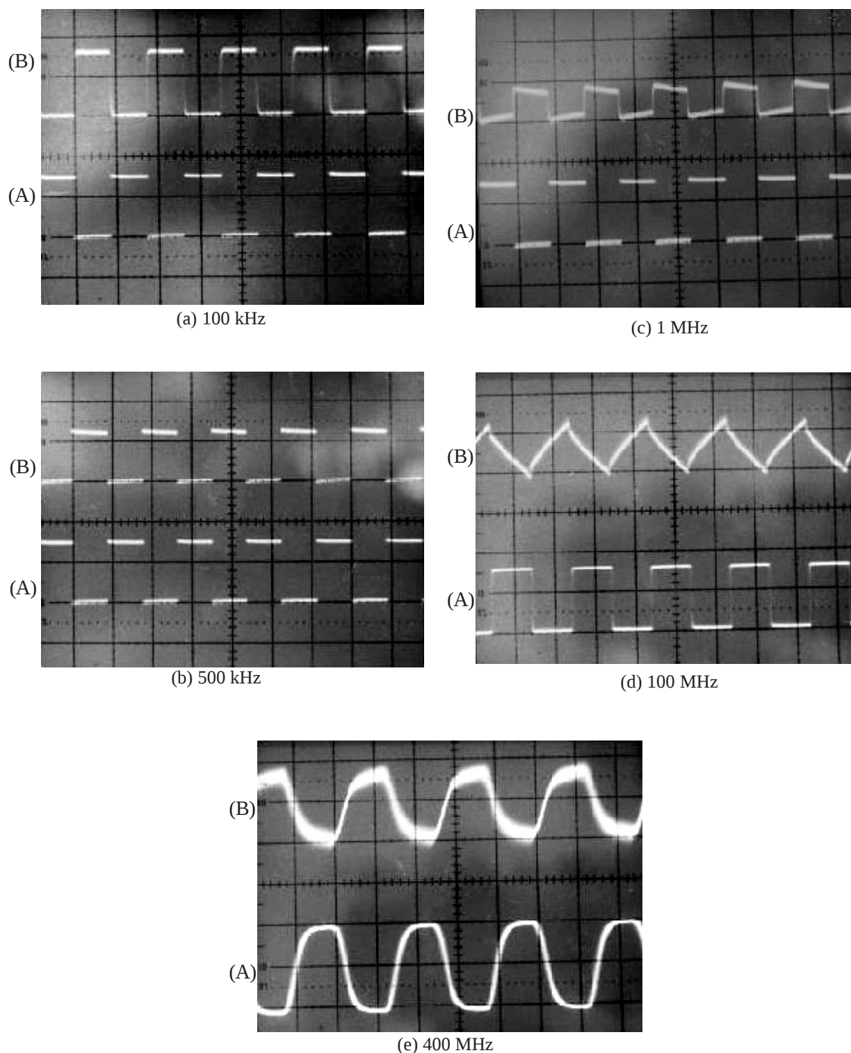
Fig. 5. Output characteristics of input wave-guide ( W_1 ) to the applied frequency (from 100 kHz to 400 MHz). (A) Input ( W_1 ), (B) Output ( W_2 ) * time/div : 500 \mu s * input : 8V
