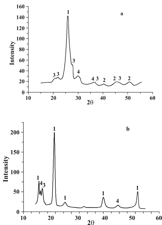
Fig. 4. XRD patterns of: a – Mo/Ni-Zn-catalyst: 1 – Ni; 2 – NiZn; 3 – \text{Ni}_3\text{Mo} ; 4 – \text{Ni}_4\text{Mo} ; b – Ti/Ni-Zn-catalyst: 1 – Ni; 2 – NiZn; 3 – NiTi; 4 – ZnO.
