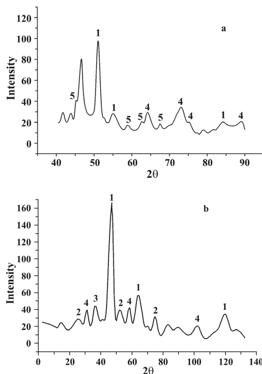
Fig. 3. XRD patterns of: a – Au/Ni-Zn-catalyst: 1 – Ni; 2 – NiZn; 3 – ZnO; 4 – Au; 5 – ZnO; b – Rh/Ni-Zn-catalyst: 1 – Ni; 2 – NiZn; 3 – ZnO; 4 – Rh.
