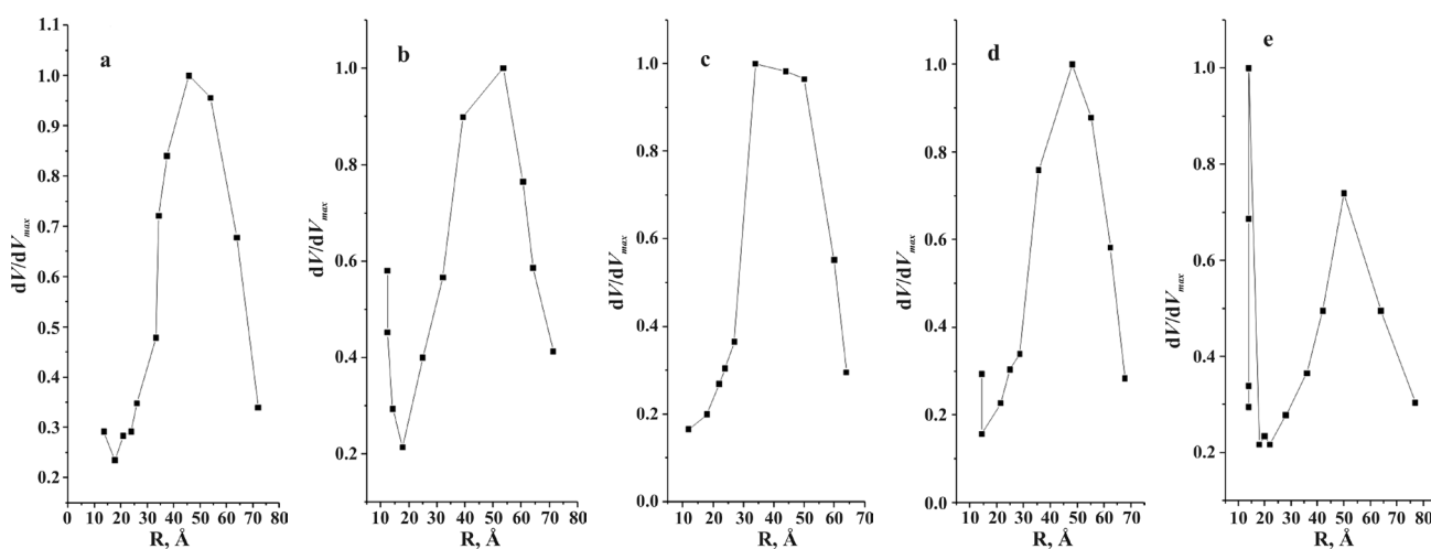
Fig. 1. Pores distribution for different Me/Ni-Zn-catalysts: a – Mo/Ni-Zn; b – Au/Ni-Zn; c – W/Ni-Zn; d – Rh/Ni-Zn; e – Ni-Zn.
