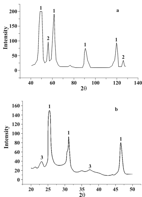
Fig. 2. XRD patterns of: a – Ni-Zn-catalyst; b – W/Ni-Zn-catalyst: 1 – Ni; 2 – NiZn; 3 – W.
