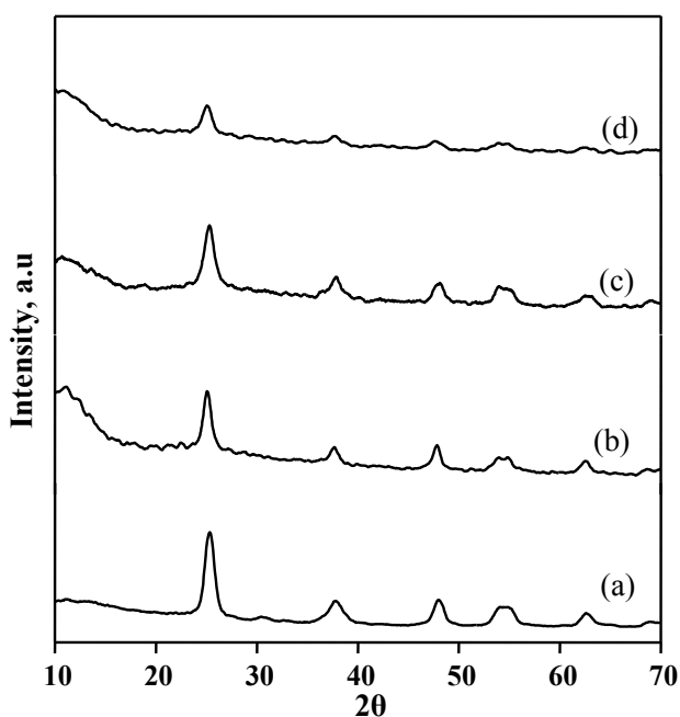
Fig. 1. X-ray diffraction profiles of (a) Ti, (b) \text{TiCr}_2 , (c) \text{TiCr}_6 and (d) \text{TiCr}_{10} .
