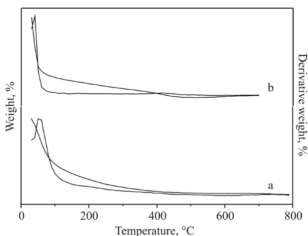
Fig. 2. TG/DTG profiles of (a) Ti and (b) \text{TiCr}_6 .
