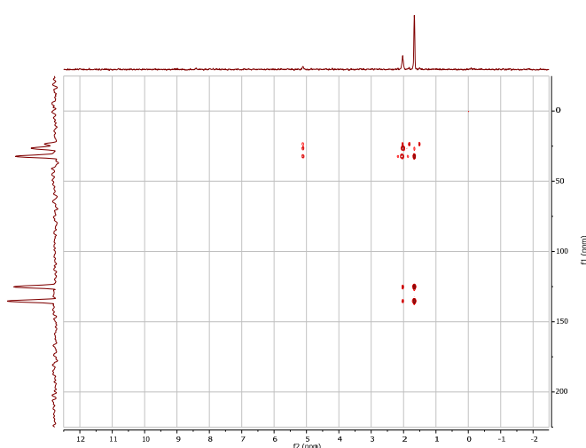
Fig. 7. HMBC ^1\text{H} - ^{13}\text{C} NMR spectra of root extracts from S. tau-saghyz Lipsch. et G.G. Bosse.
