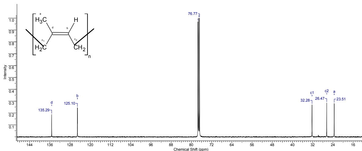
Fig. 3. ^{13}\text{C} NMR spectra of root extracts from S. tau-saghyz Lipsch. et G.G. Bosse.
