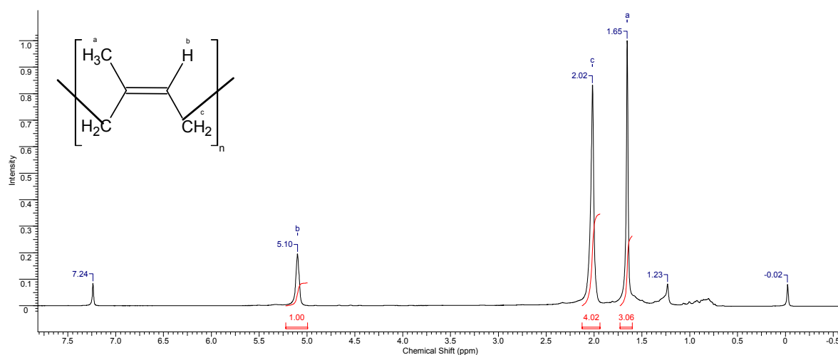
Fig. 2. ^1\text{H} NMR spectra of rubber in root extracts of S. tau-saghyz Lipsch. et G.G. Bosse plants.
