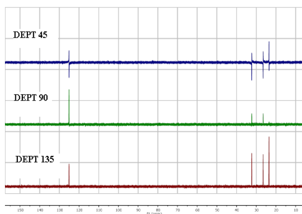
Fig. 4. DEPT spectra of root extracts from S. tau-saghyz Lipsch. et G.G. Bosse.
