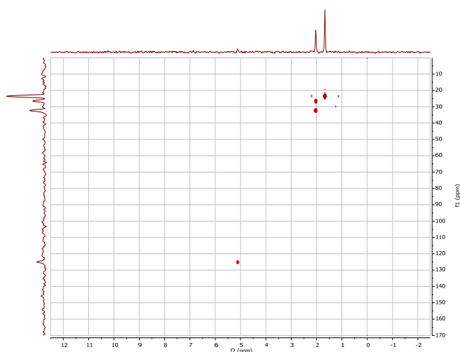
Fig. 6. HMBC ^1\text{H} - ^{13}\text{C} NMR spectra of root extracts from rubber producing plant S. tau-saghyz .
