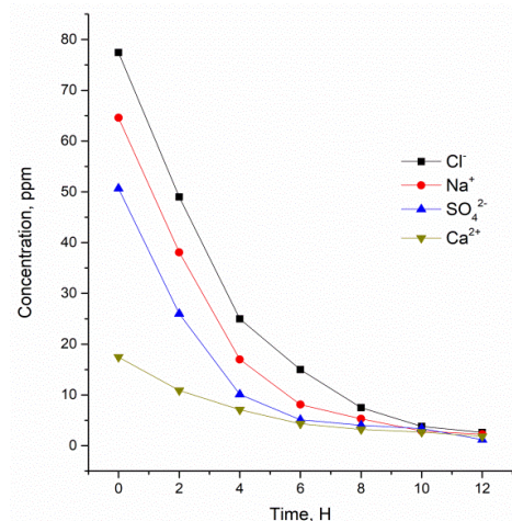
Fig. 2. Deionization of diatomite.
