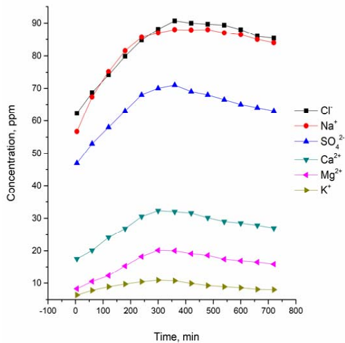
Fig. 1. Release of ions from diatomite.
