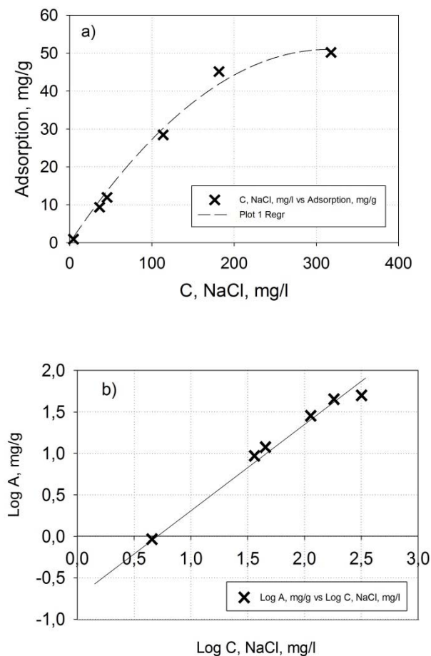
Fig. 4. Isotherm of NaCl adsorption on deionized diatomite; (a) is the equilibrium adsorption value (mg/g), C-equilibrium concentration (a) mg/l, (b) double-logarithmic (log-log) scale. The mass ratio of adsorbent/solution is 1/100; A concentration range of sodium chloride C_0 = 3\text{--}350 mg/l.
